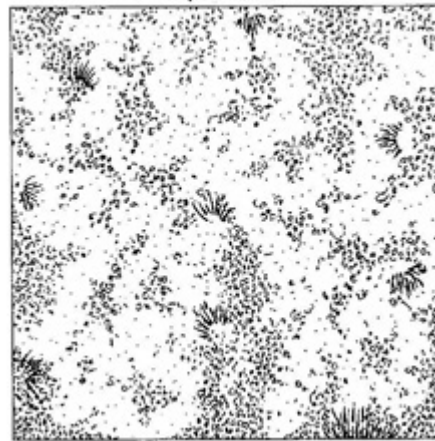
Coquina Texture
